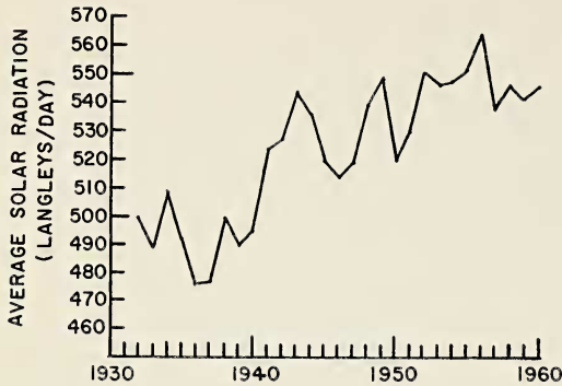
FIG. 9. Solar radiation at Makiki, 1932-60.
